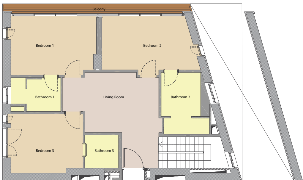
4 th Floor
